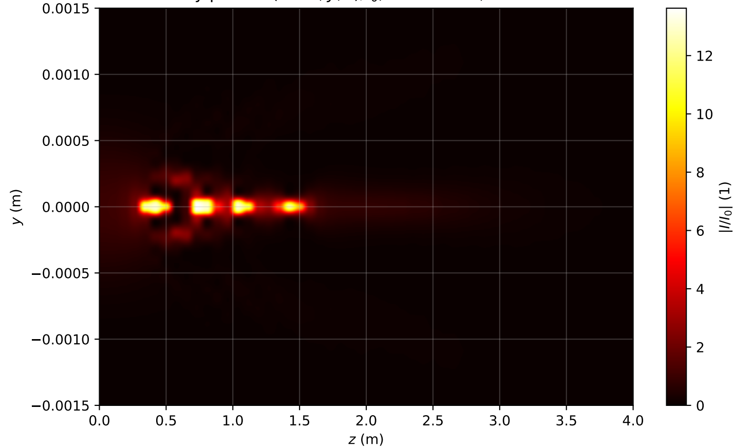
Intensity profile I(x=0, y, z)/I_0 , P_{in}=8.5P_{cr} , artificial time
